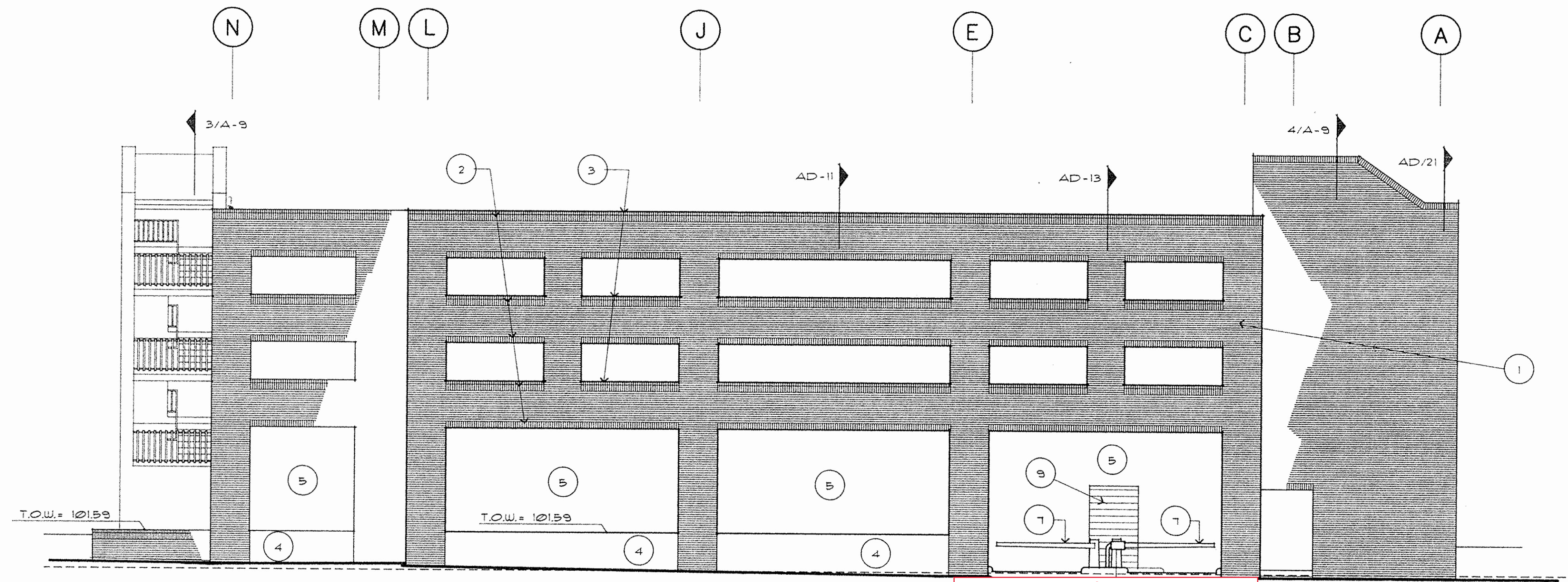
WEST ELEVATION
