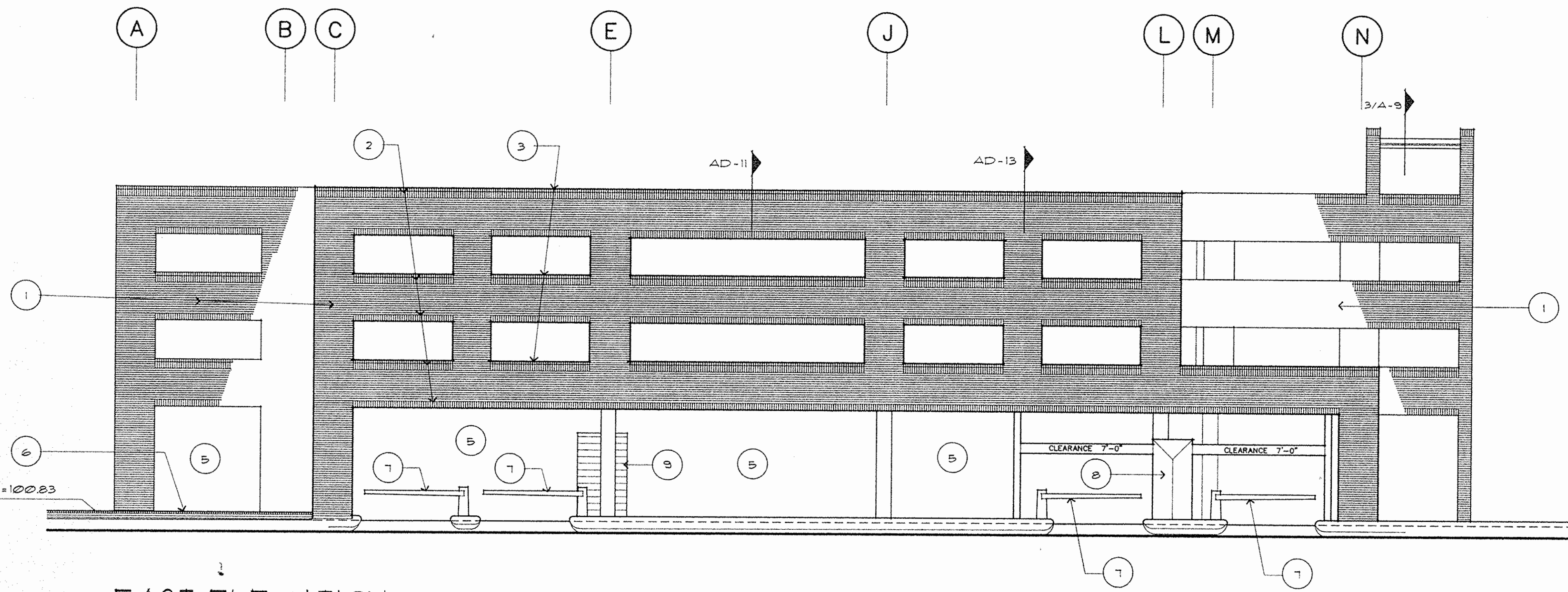
EAST ELEVATION
